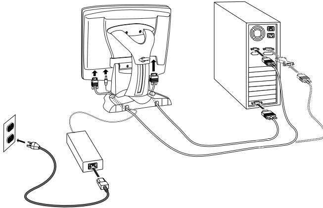
Figure 7 Connecting the M150 Cables to your Computer
