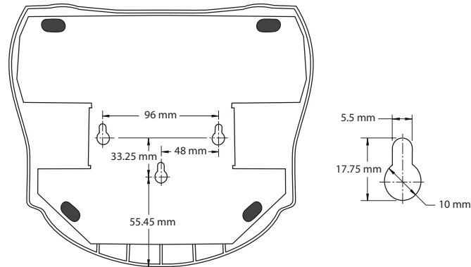
Figure 2 Keyhole Mounting Slots
